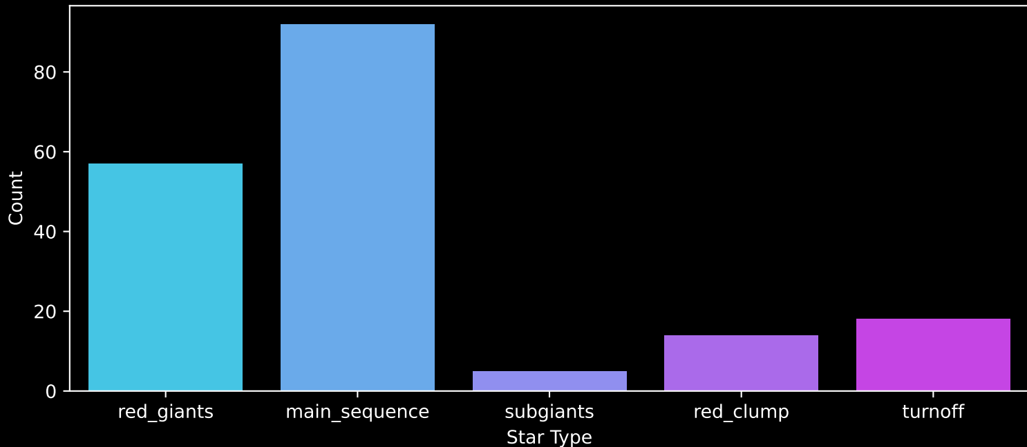
APOGEE DR17 Field: [201+27_MGA] Count plot of Star Type
