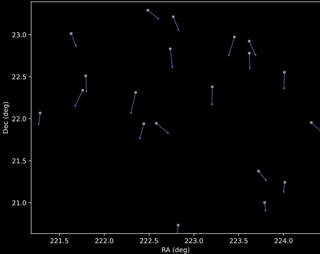
APOGEE DR17 Cluster 8 Proper Motion Vectors (n=20)
