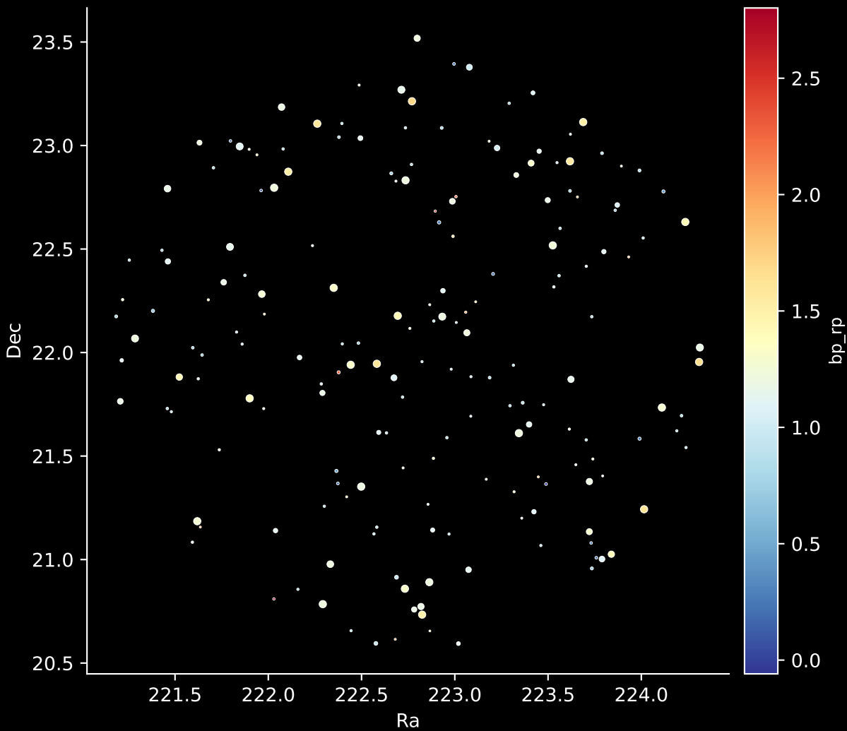
APOGEE DR17 Field: [201+27_MGA] Stars: 186
