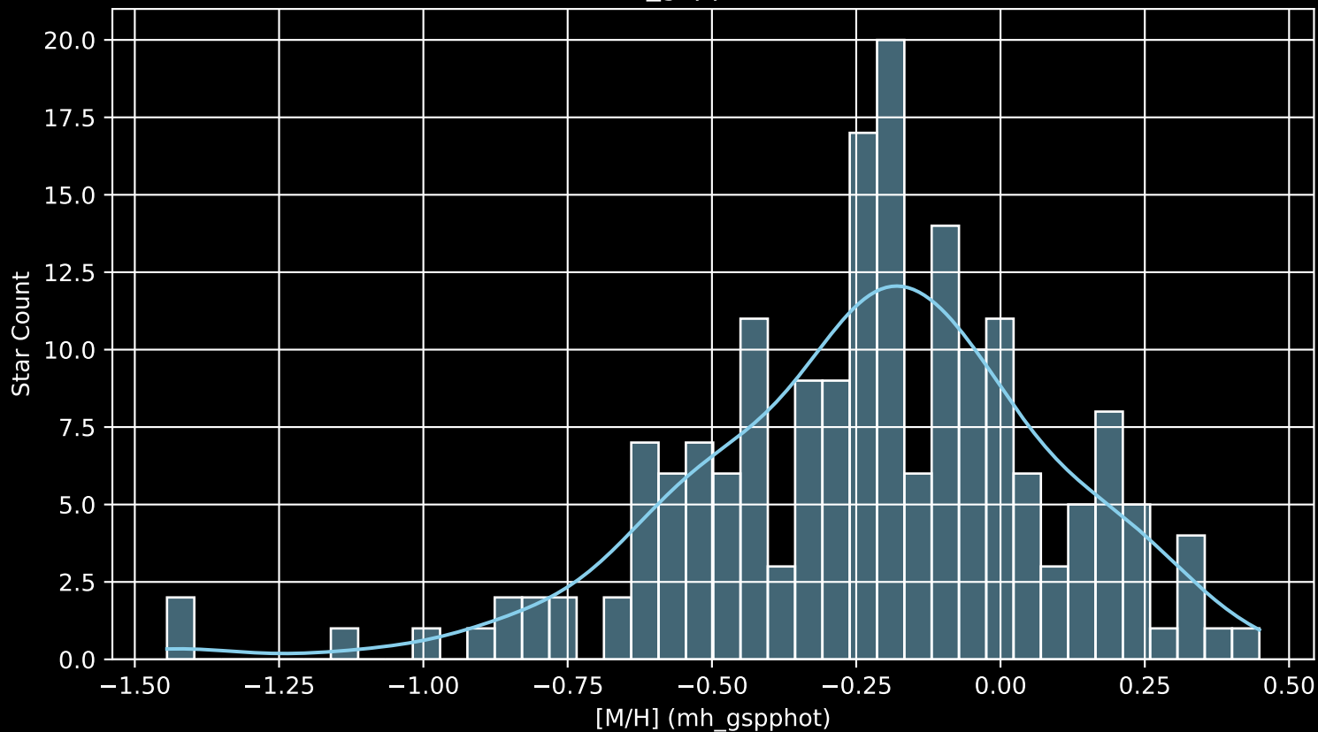
APOGEE DR17 Field: [201+27_MGA [M/H] (mh_gspphot) (n= 183)
