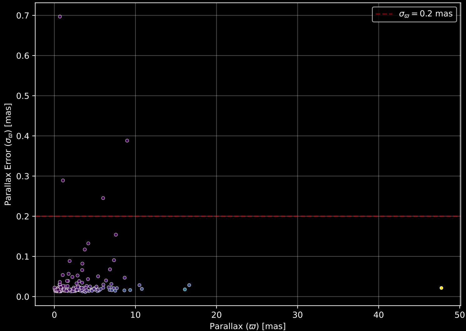
APOGEE DR17 Field: [201+27_MGA] Parallax Quality (n= 186)
