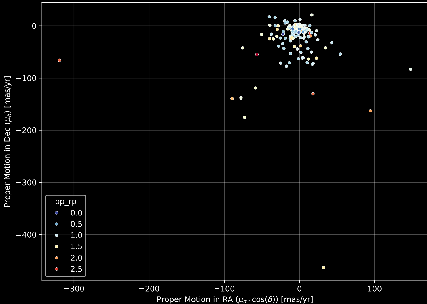
APOGEE DR17 Field: [201+27_MGA] Proper Motion Diagram (n= 186)
