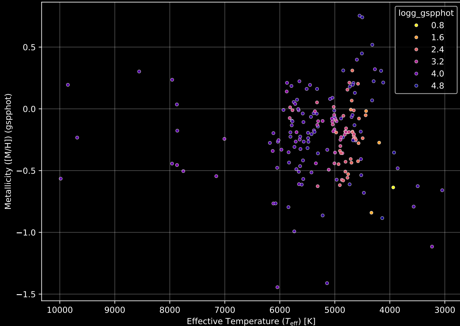
APOGEE DR17 Field: [201+27_MGA] Stellar Population Parameters (n= 186)
