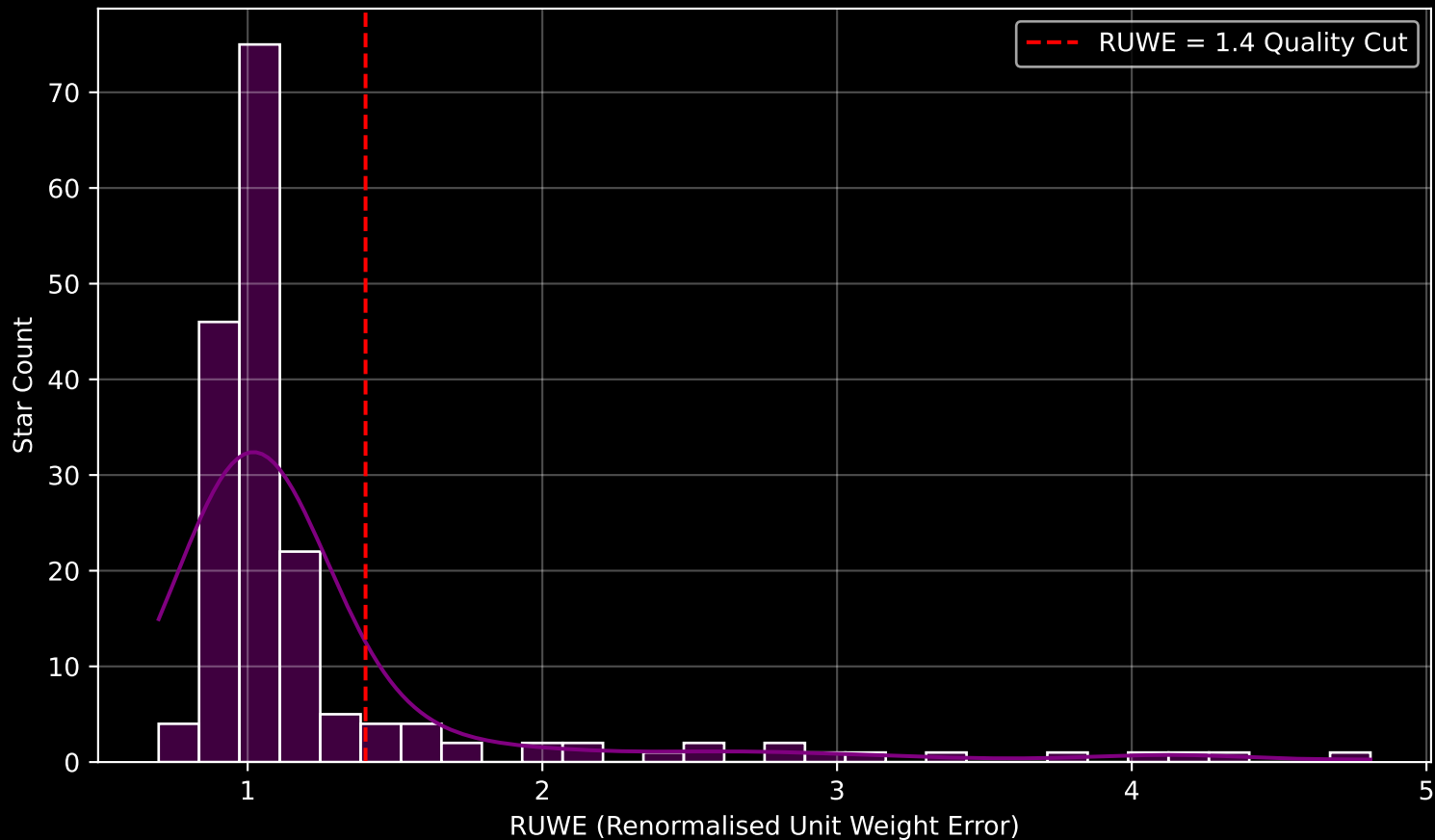
GAPOGEE DR17 Field [201+27_MGA] RUWE Distribution (n= 179)
